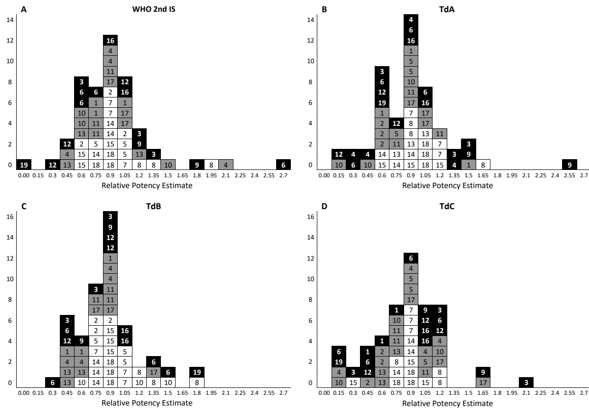
Figure 4 – Histograms of relative potency (RP) estimates of test samples
